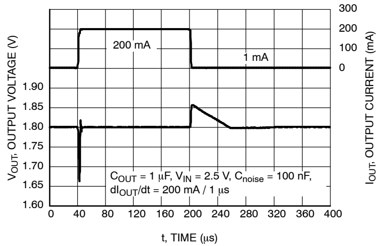
Figure 27. Load Transient Response, V_{\text{OUT}} = 1.8 \text{ V} , C_{\text{OUT}} = 1 \mu\text{F} , C_{\text{noise}} = 100 \text{ nF}
