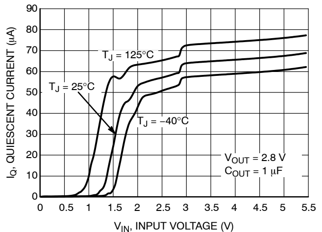
Figure 50. Quiescent Current vs. Input Voltage, V_{OUT} = 2.8\text{ V} , C_{OUT} = 1\ \mu\text{F}
