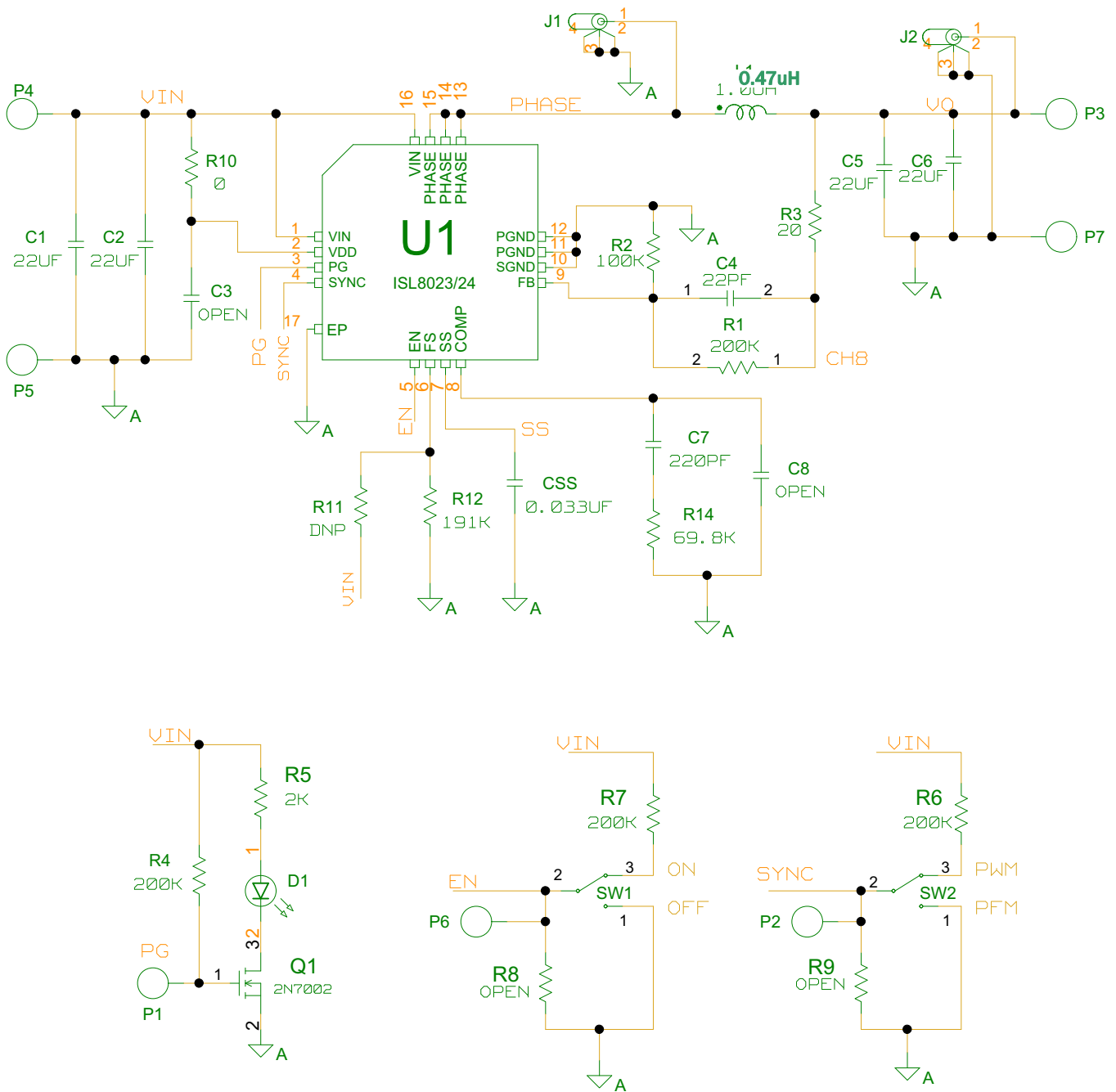
FIGURE 6. SCHEMATIC
